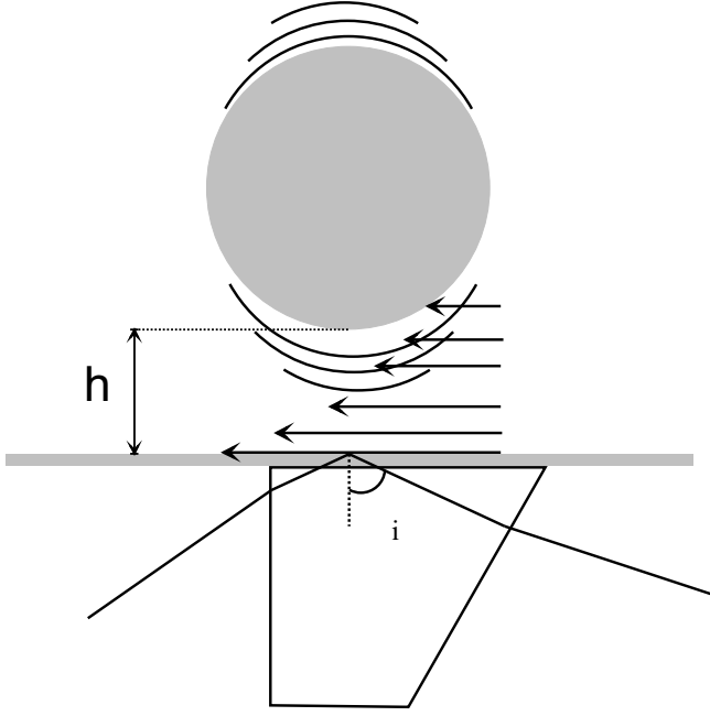
Fig. 1 Sketch of the evanescent wave optics.
