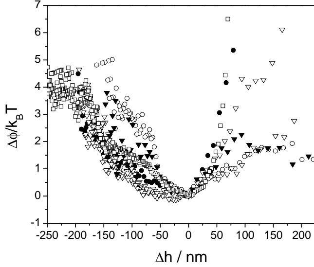
Fig. 6 Various interaction profiles of polystyrene latex spheres with PEM. Circles: 4.54 \mu\text{m} PSS spheres above eight PDADMAC/PSS double layers; Down Triangles: 4.54 \mu\text{m} PSS spheres above one PDADMAC/PSS double layer; Square: 2.92 \mu\text{m} PSA spheres above a PEI/PSS/PDADMAC assembly. Open symbols refer to a nominal Debye length of \kappa^{-1} \approx 30 nm, full symbols to \kappa^{-1} \approx 14 nm.
