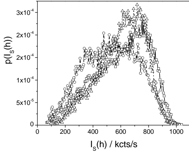
Fig. 3 Intensity histograms from TIRM experiments on PSA spheres floating above a glass surface coated with a single PEI-layer. Different line types represent different spheres at different locations.
